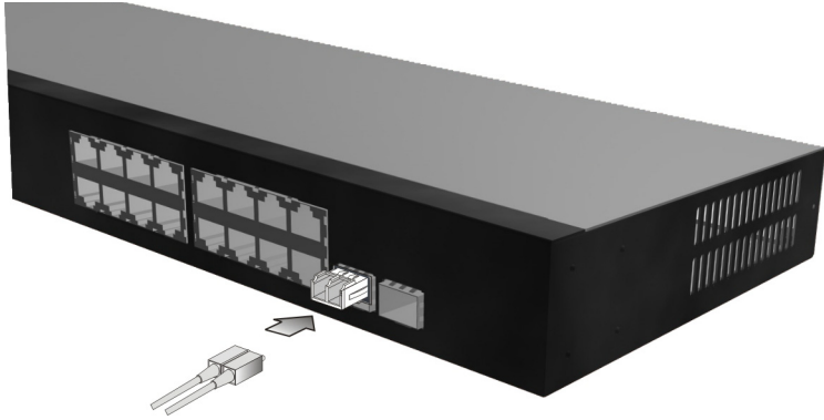
Figure 17: Making Fiber Port Connections
