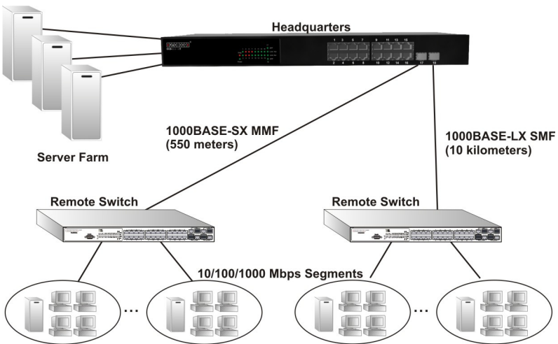
Figure 7: Remote Connections with Fiber Cable
