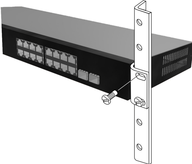
Figure 11: Installing the Switch in a Rack
