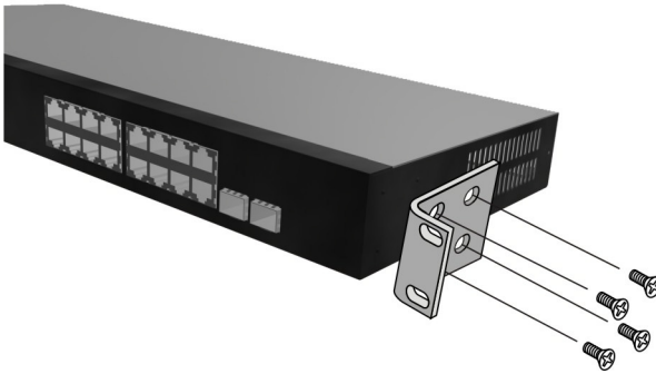
Figure 10: Attaching the Brackets
