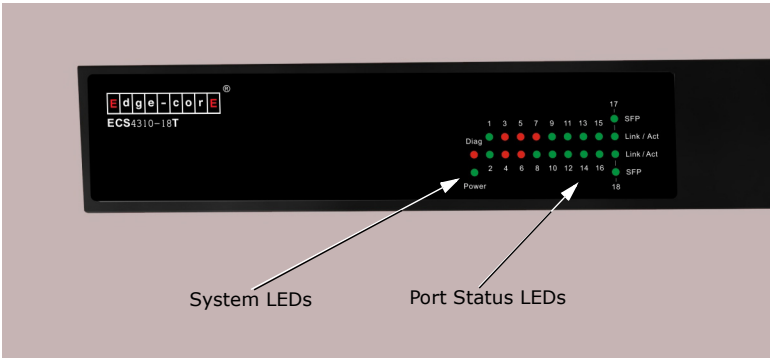
Figure 3: Port and System LEDs
