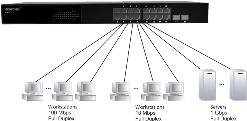
Figure 5: Collapsed Backbone
