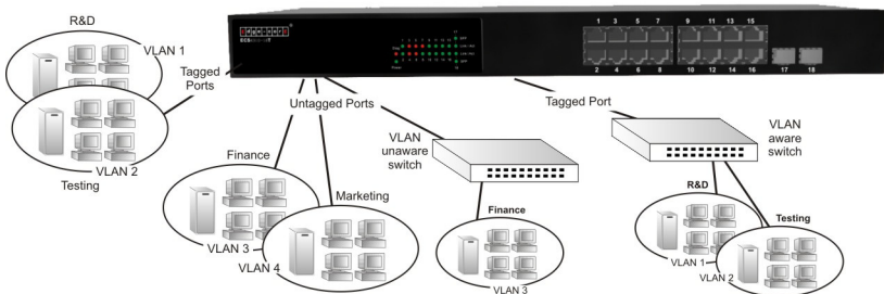
Figure 8: Making VLAN Connections
